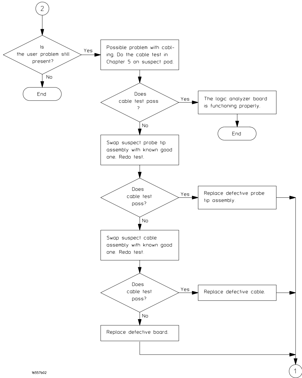
Troubleshooting Flowchart 2
