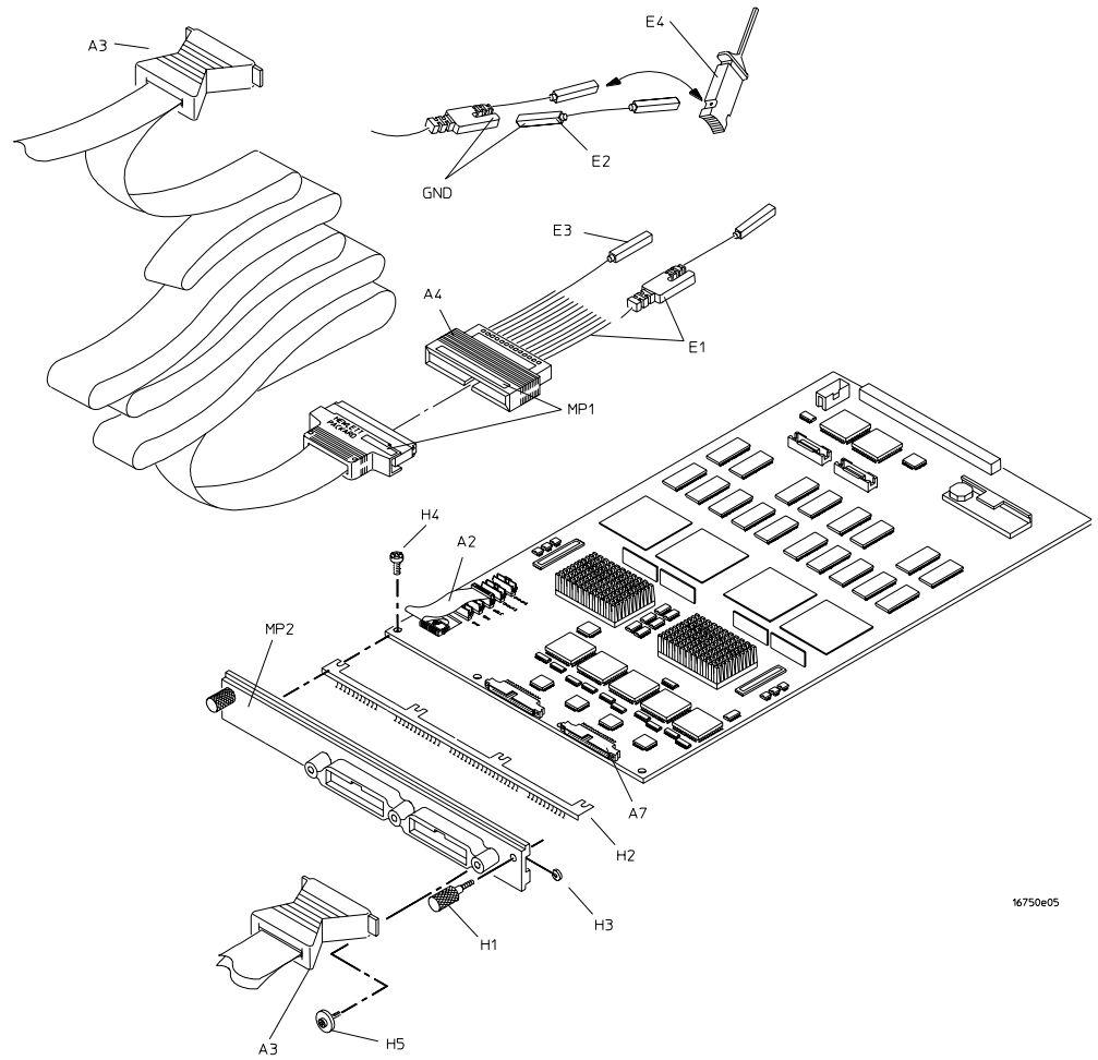
Exploded view of the 16750/51/52B logic analyzer
